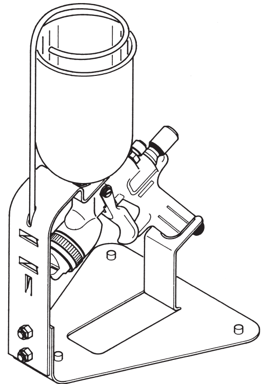
Typical Gun Stand Arrangement with Gravity Feed Gun
